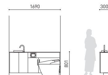
lavatory counter plan
