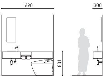
lavatory counter plan
