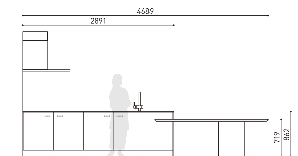
kitchen plan
