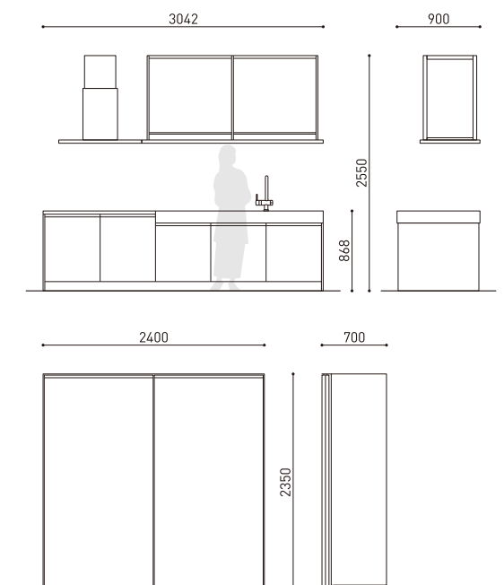
kitchen plan
