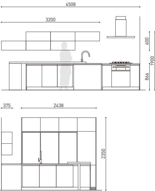
kitchen plan
