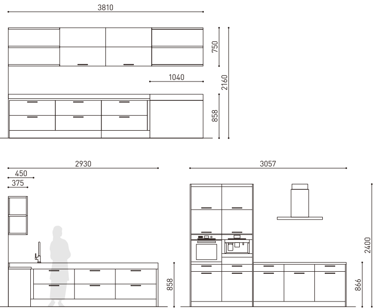
kitchen plan
