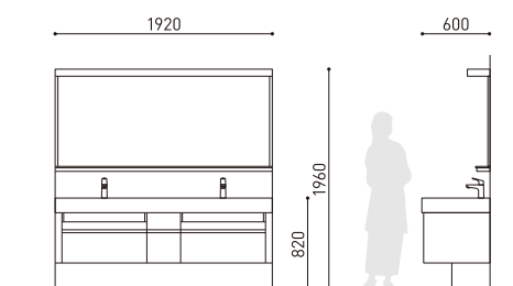
washbasin plan
