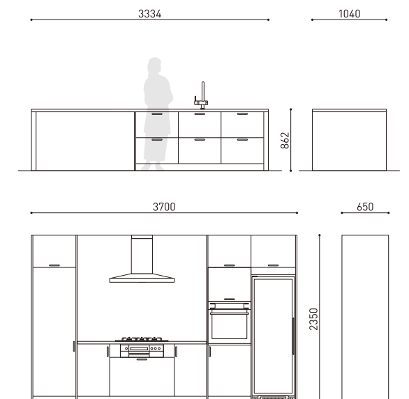
kitchen plan
