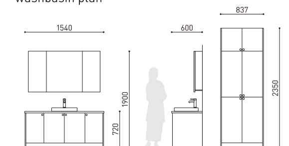
washbasin plan
