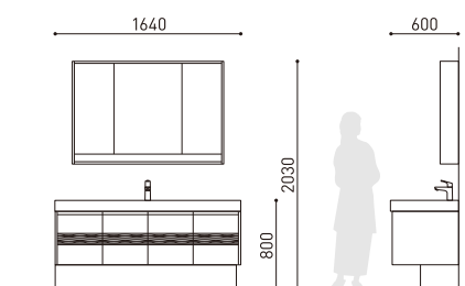
washbasin plan
