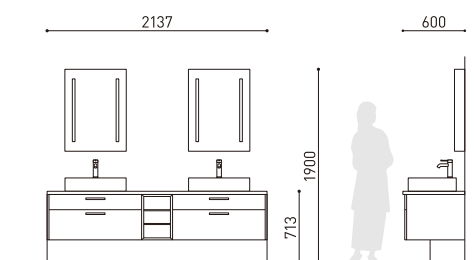
washbasin plan
