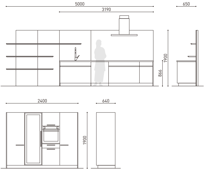
kitchen plan
