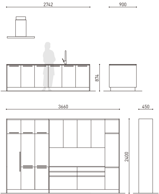
kitchen plan
